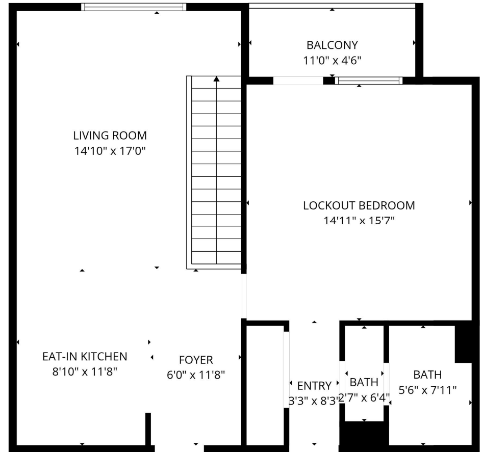
2nd floor
