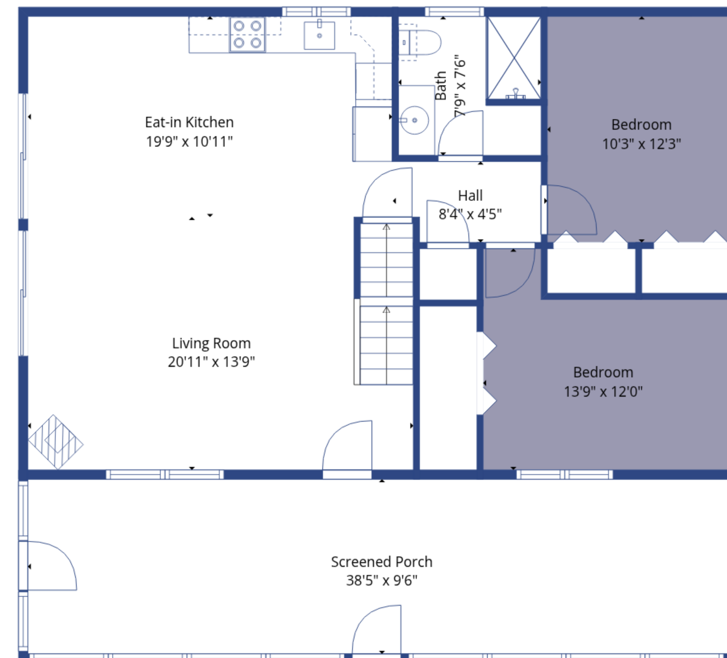
1st Floor
