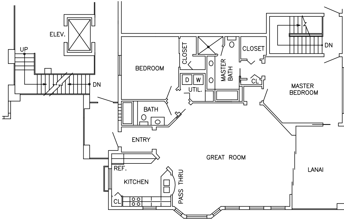
TYPICAL UNIT A (UNIT B MIRROR IMAGE)
