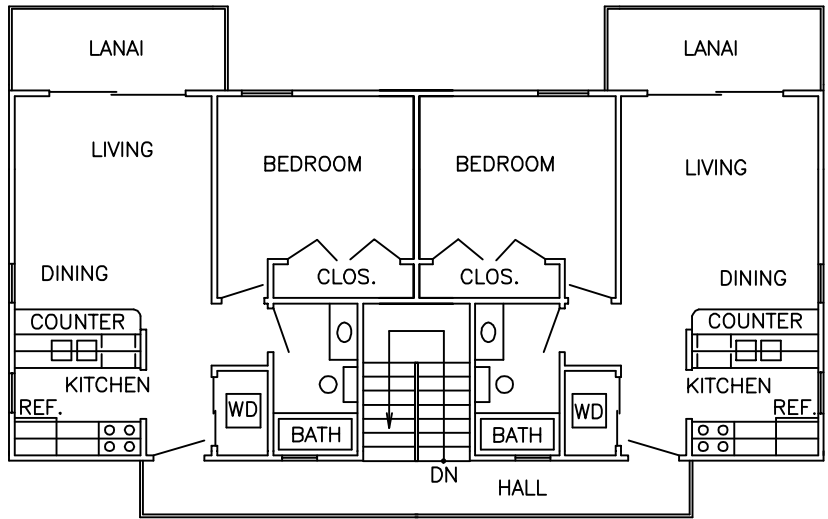
FLOOR PLAN UNIT 11 & 13
