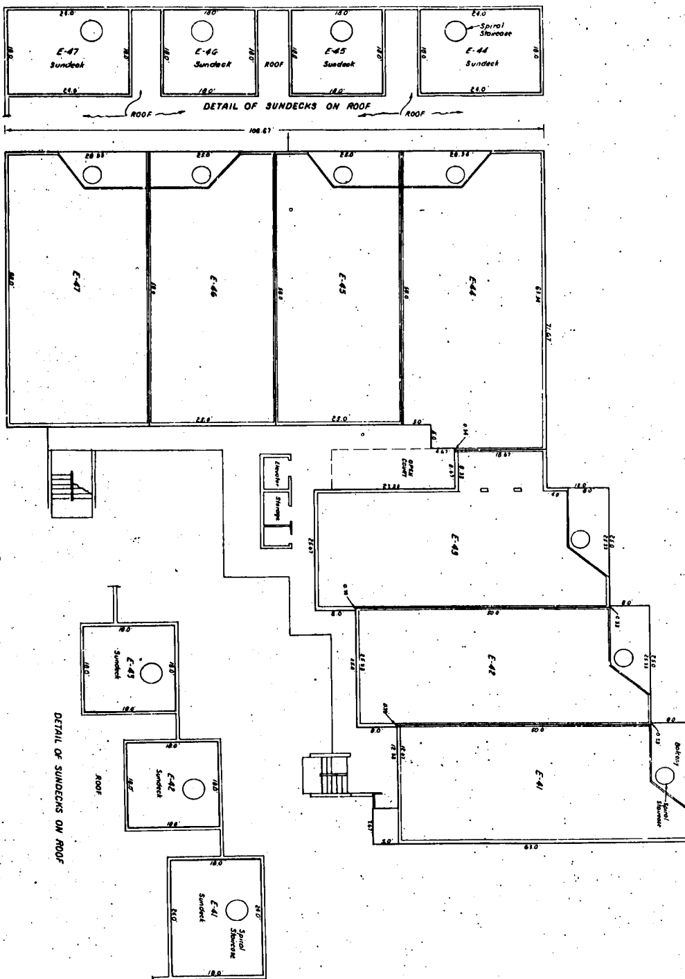
BLDG. 2 FOURTH FLOOR PLAN AND ROOF SUNDECKS
