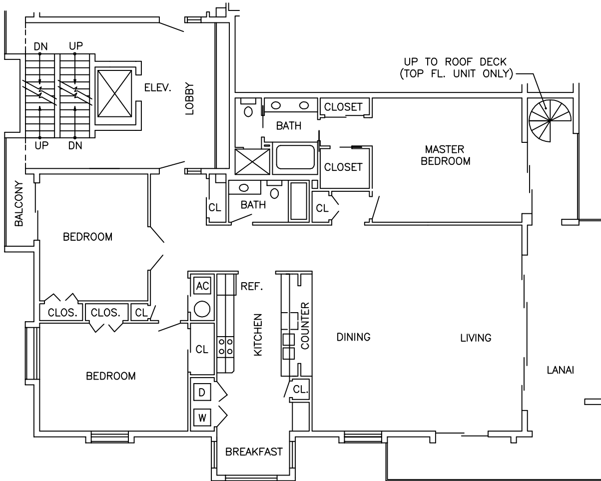
TYPICAL UNITS 2, 4 & 6 (UNITS 1, 3 & 5 MIRROR IMAGE)
