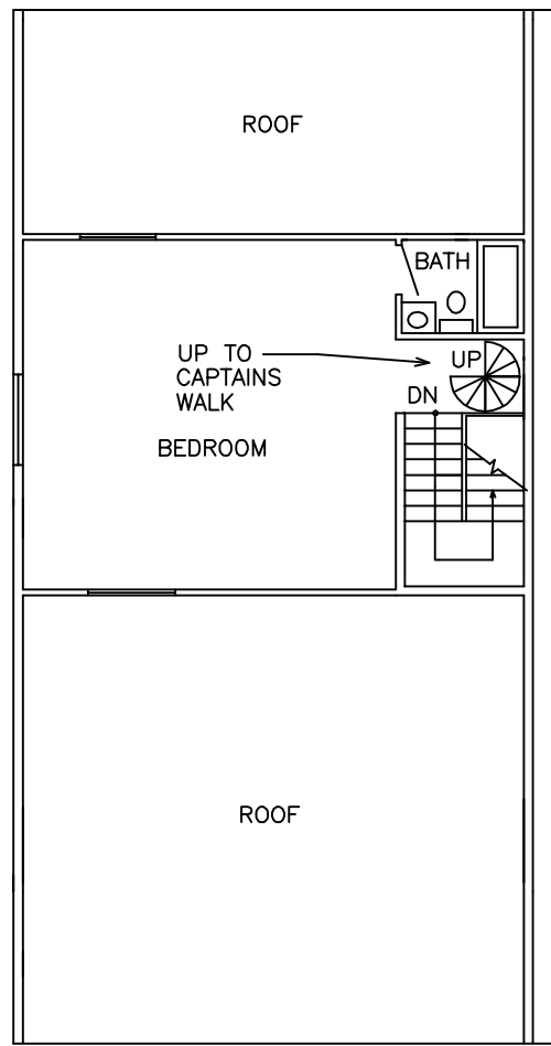
LOFT PLAN UNITS 16,17,18 & 19
