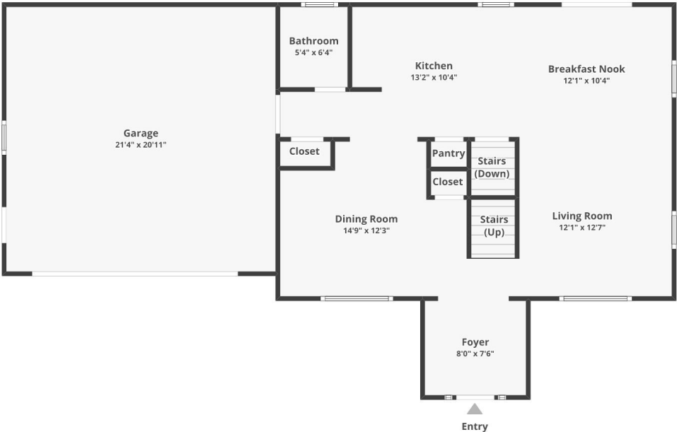
FLOOR 1
