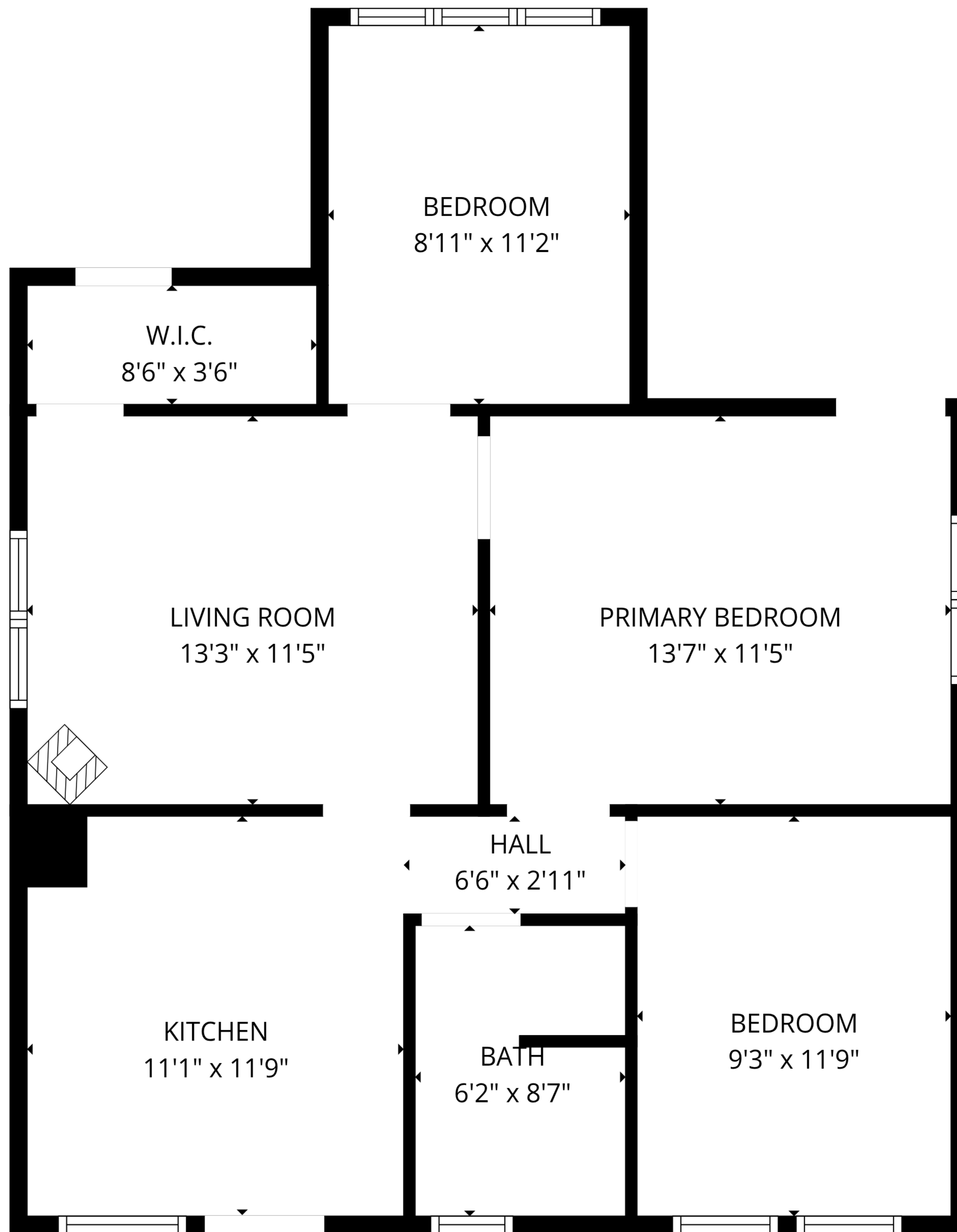
SECOND FLOOR UNIT
