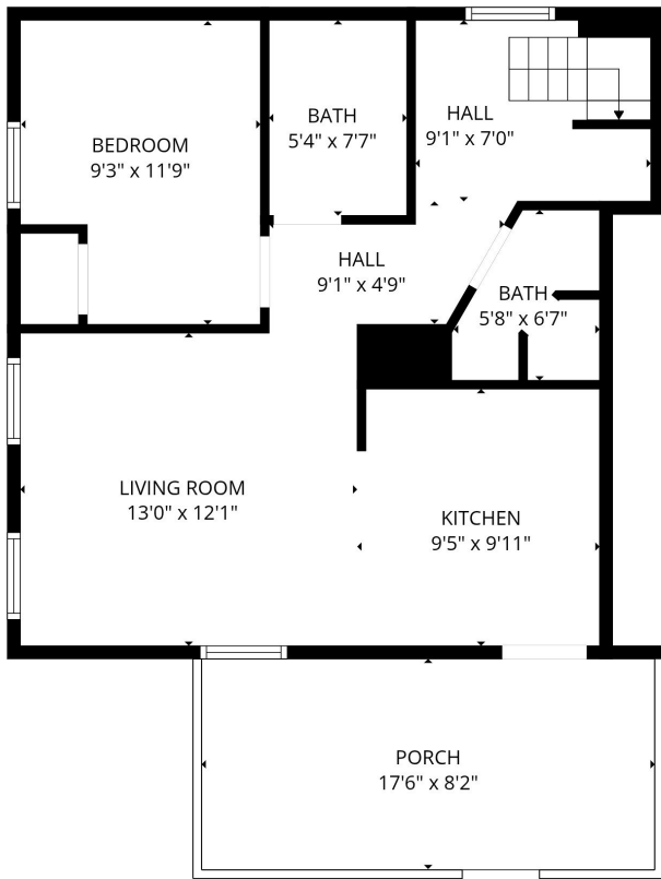
1st floor
