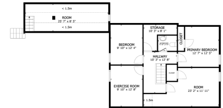
FLOOR 3
