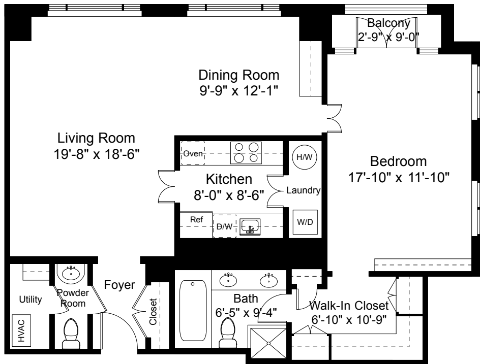
Unit 302 Floor Plan Ceiling Height = 8'-0"
