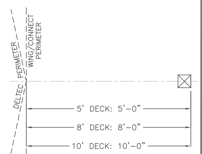
DETAIL 2-C TYPICAL DECK-POST LOCATION DIMENSIONS (UNLESS OTHERWISE NOTED) SCALE: 1/2"=1'-0"
