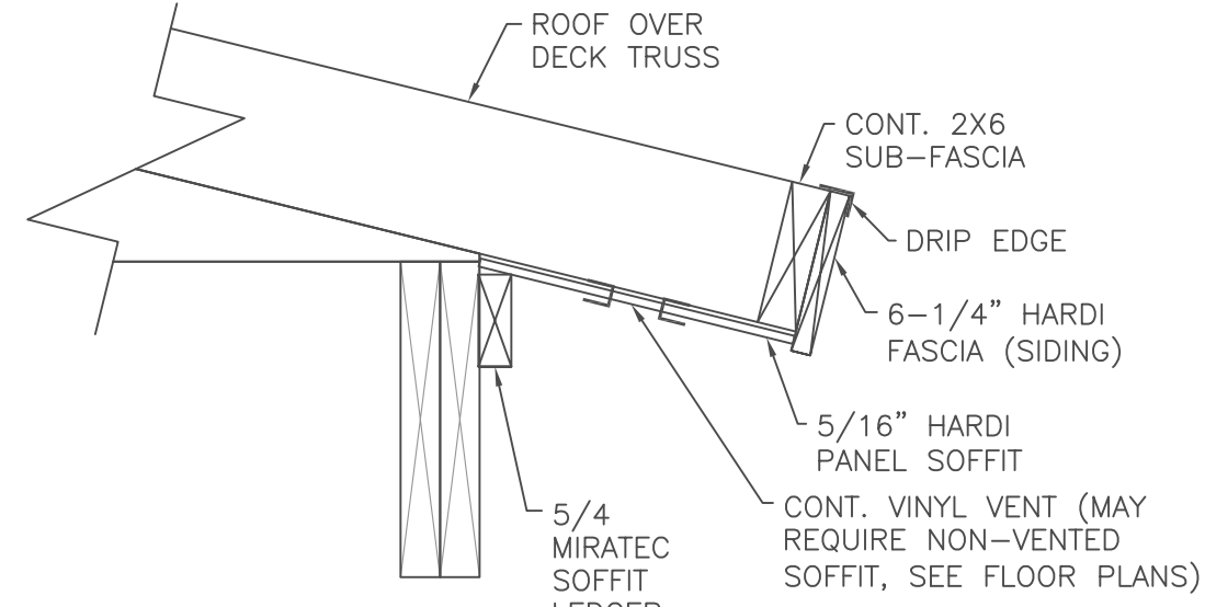
DETAIL 9-A1 HARDI SOFFIT DETAIL SCALE: 1-1/2"=1'-0"
