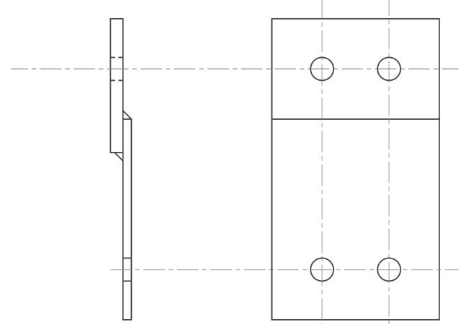
DETAIL 9-K DECK POST/DECK BEAM CONNECTOR PLATE (2 REQUIRED) DECK BEAM DECK ROOF POST (2 REQUIRED INVERTED) SCALE: 3"=1'-0"
