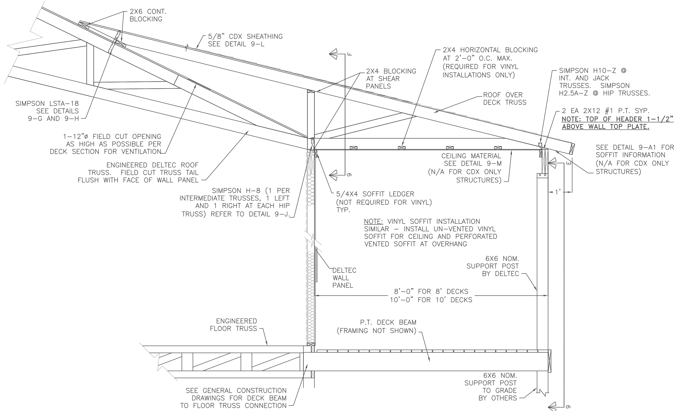
SECTION 9-A ROOF SECTION TAKEN AT HIP SCALE: 1/2"=1'-0"
