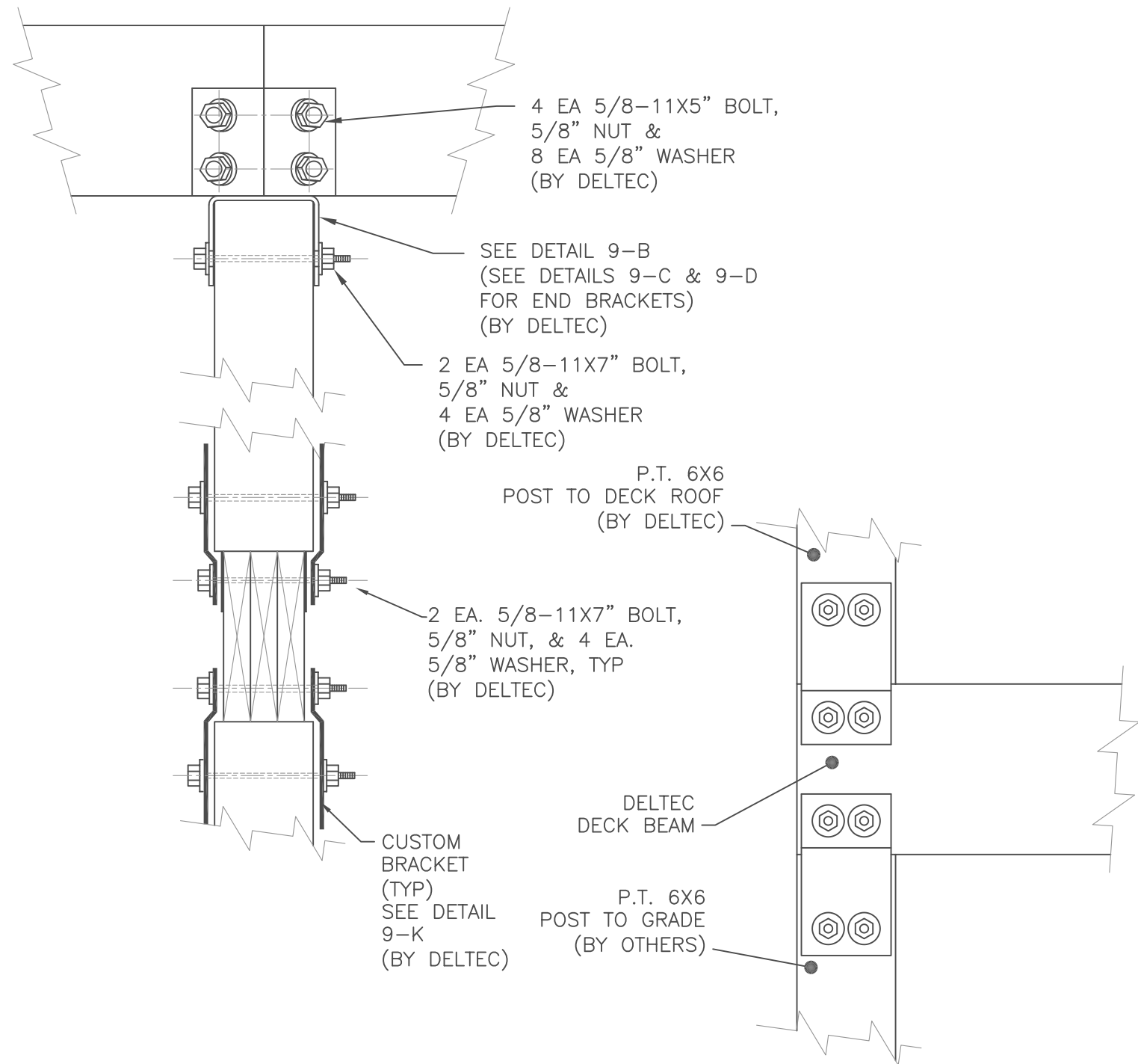
SECTION 9-E
