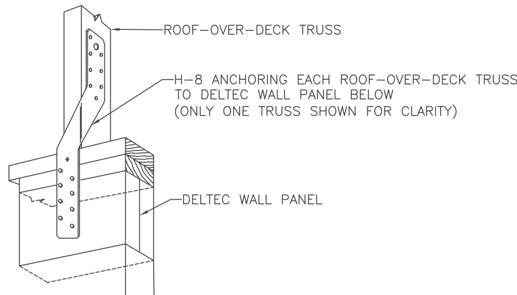
DETAIL 9-J SIMPSON H8 ATTACHMENT TO WALL AT DECK ROOF TRUSSES NTS
