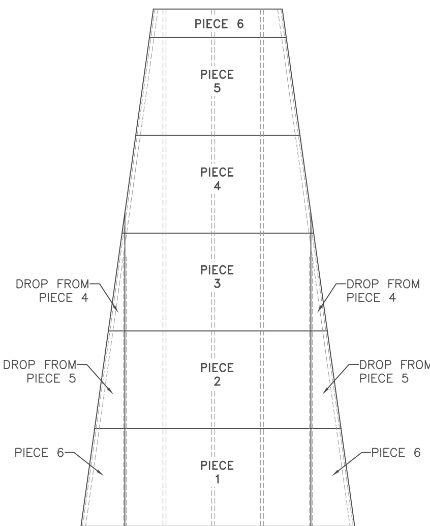
DETAIL 9-L 10' ROOF OVER DECK SHEATHING LAYOUT SCALE: 1/4"=1'-0"
