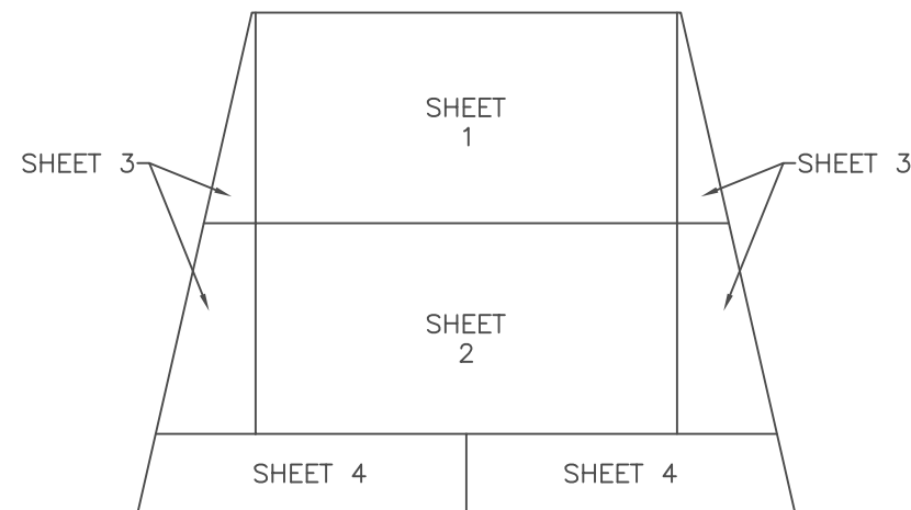
DETAIL 9-M 10' ROOF OVER DECK CEILING LAYOUT (4 SHEETS PER BAY) SCALE: 1/4"=1'-0"
