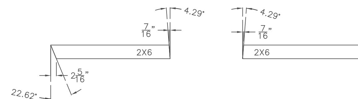
DETAIL 8-A 8' LADDER RAFTER 3'-9" OH SCALE: 1/2"=1' (2 REQUIRED)
