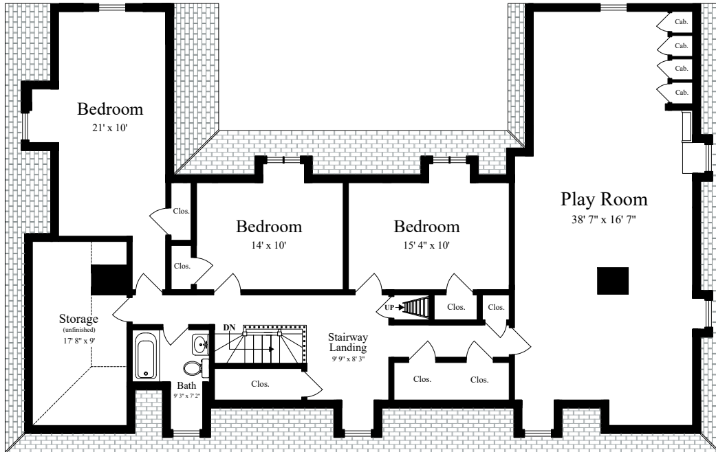
THIRD FLOOR (ceiling = 7' 6")
