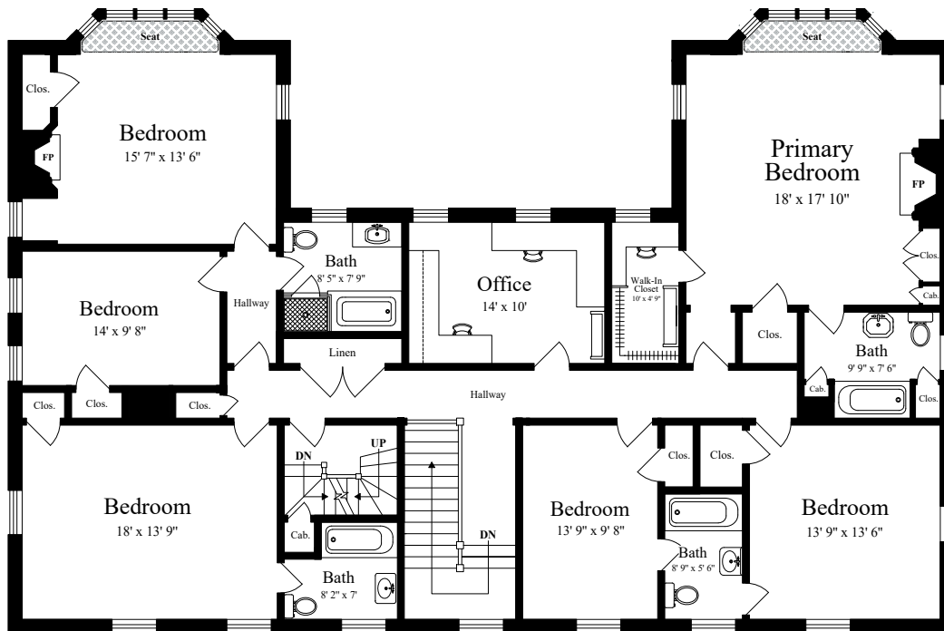
SECOND FLOOR (ceiling = 7' 8")
