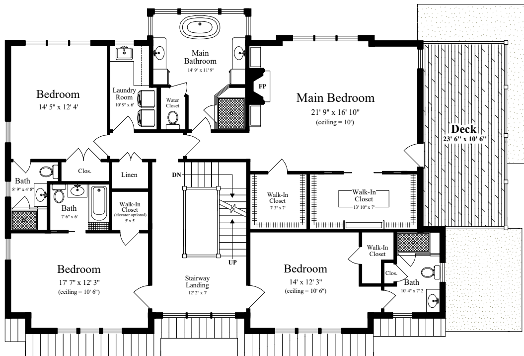
SECOND FLOOR (ceiling = 9')
