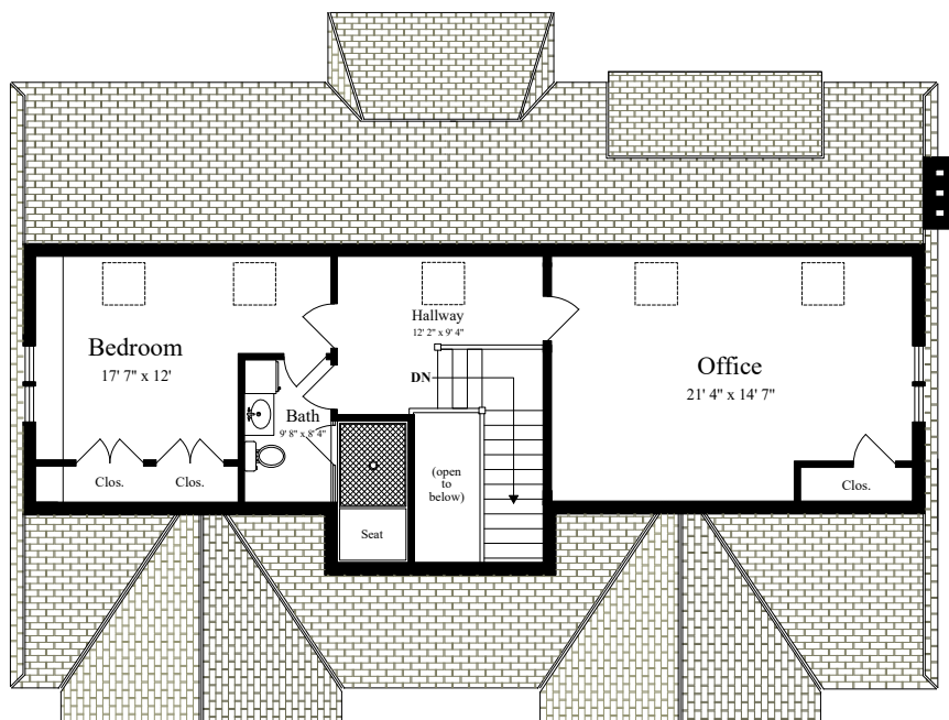
THIRD FLOOR (Cathedral Ceiling)
