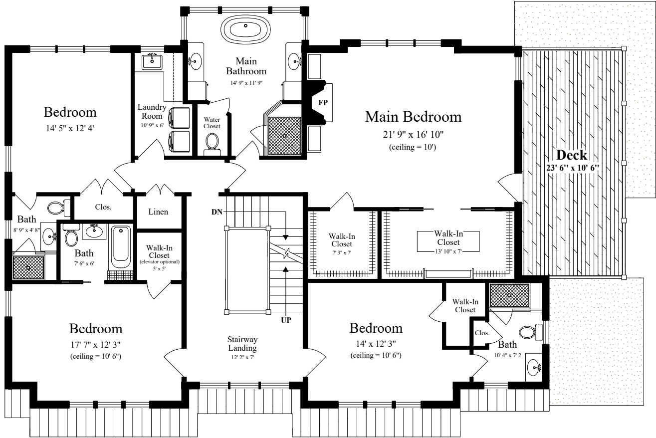
SECOND FLOOR (ceiling = 9')
