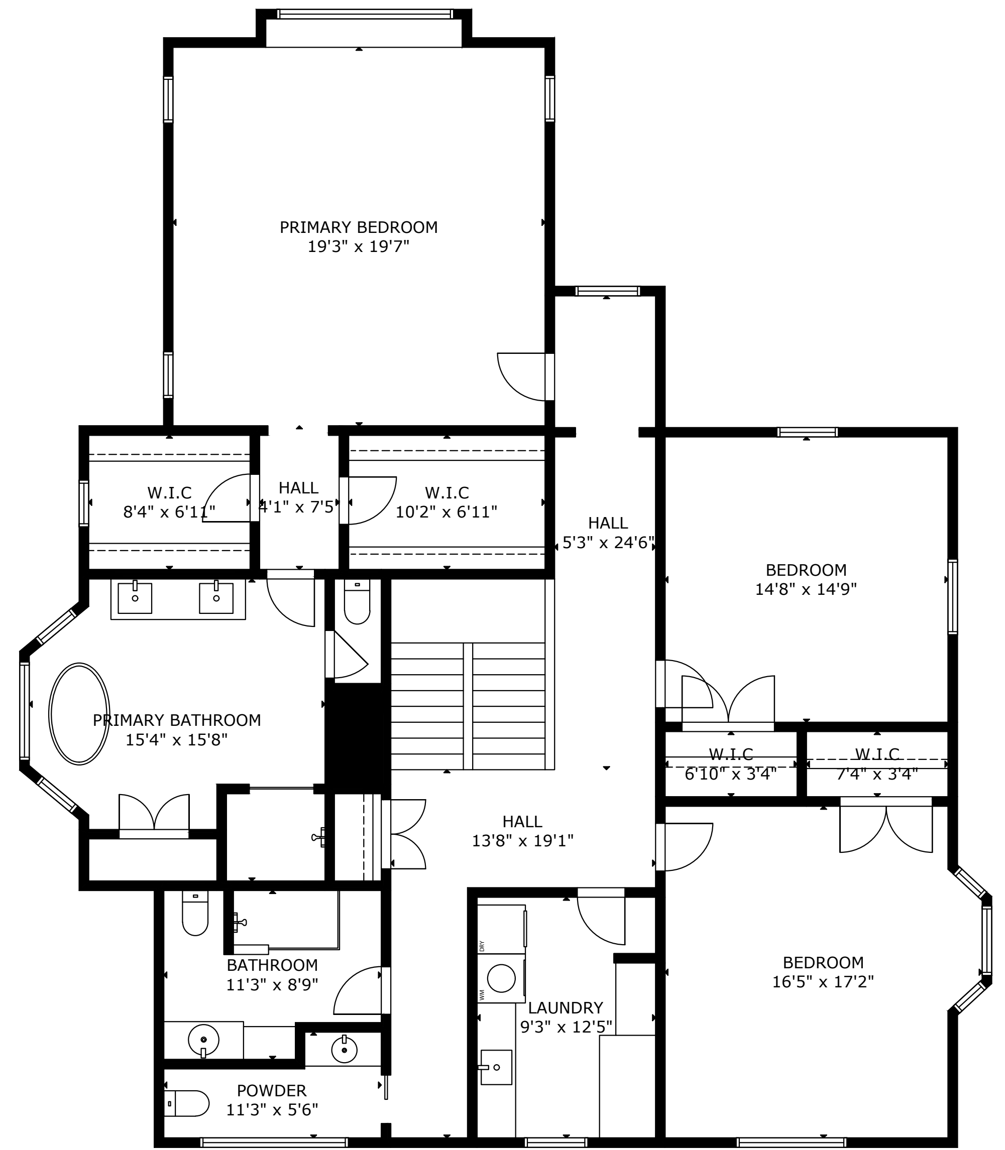
FLOOR 2
