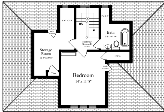
THIRD FLOOR (ceiling = 7' 6")
