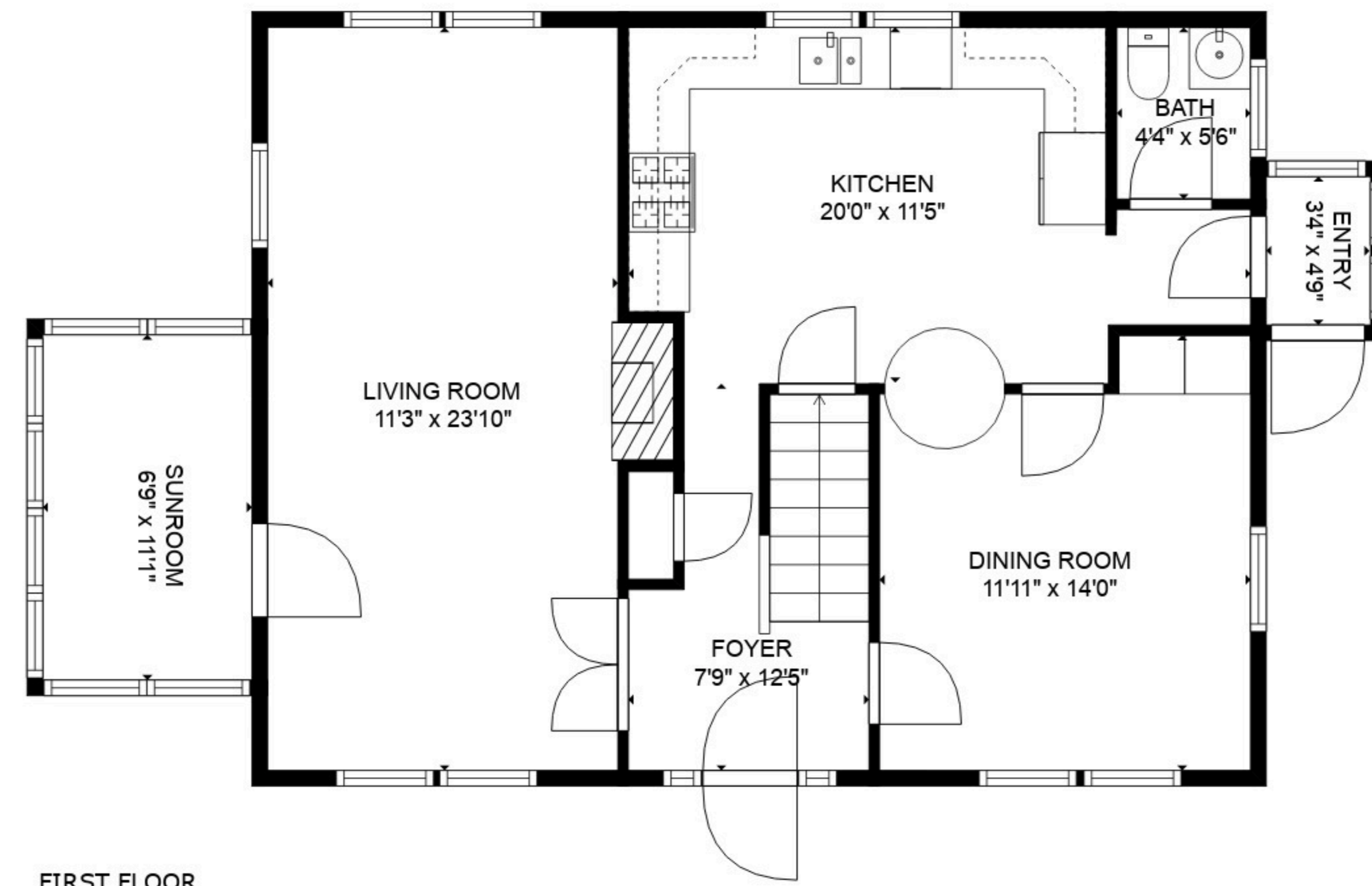
FIRST FLOOR
