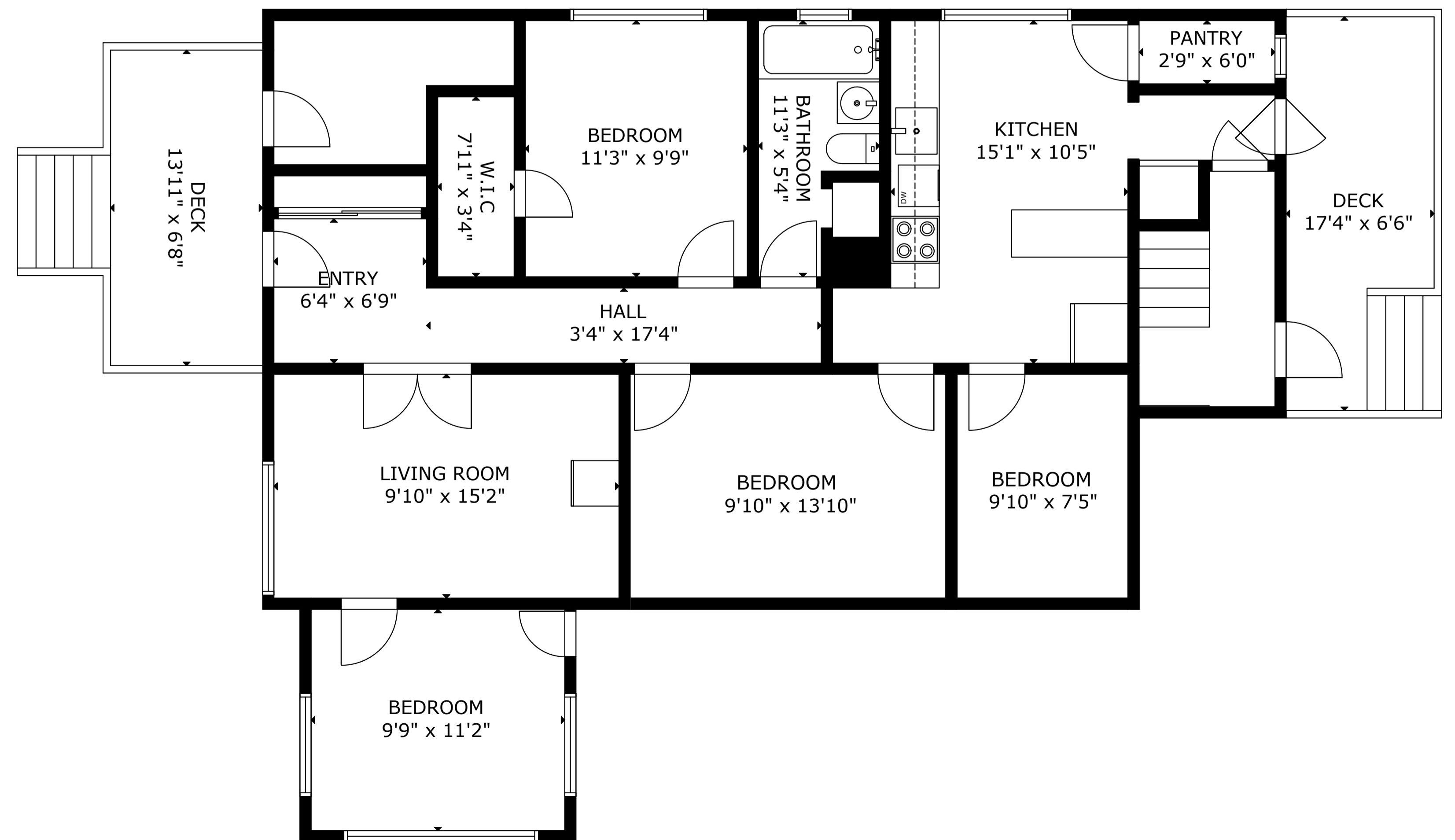
FIRST FLOOR
