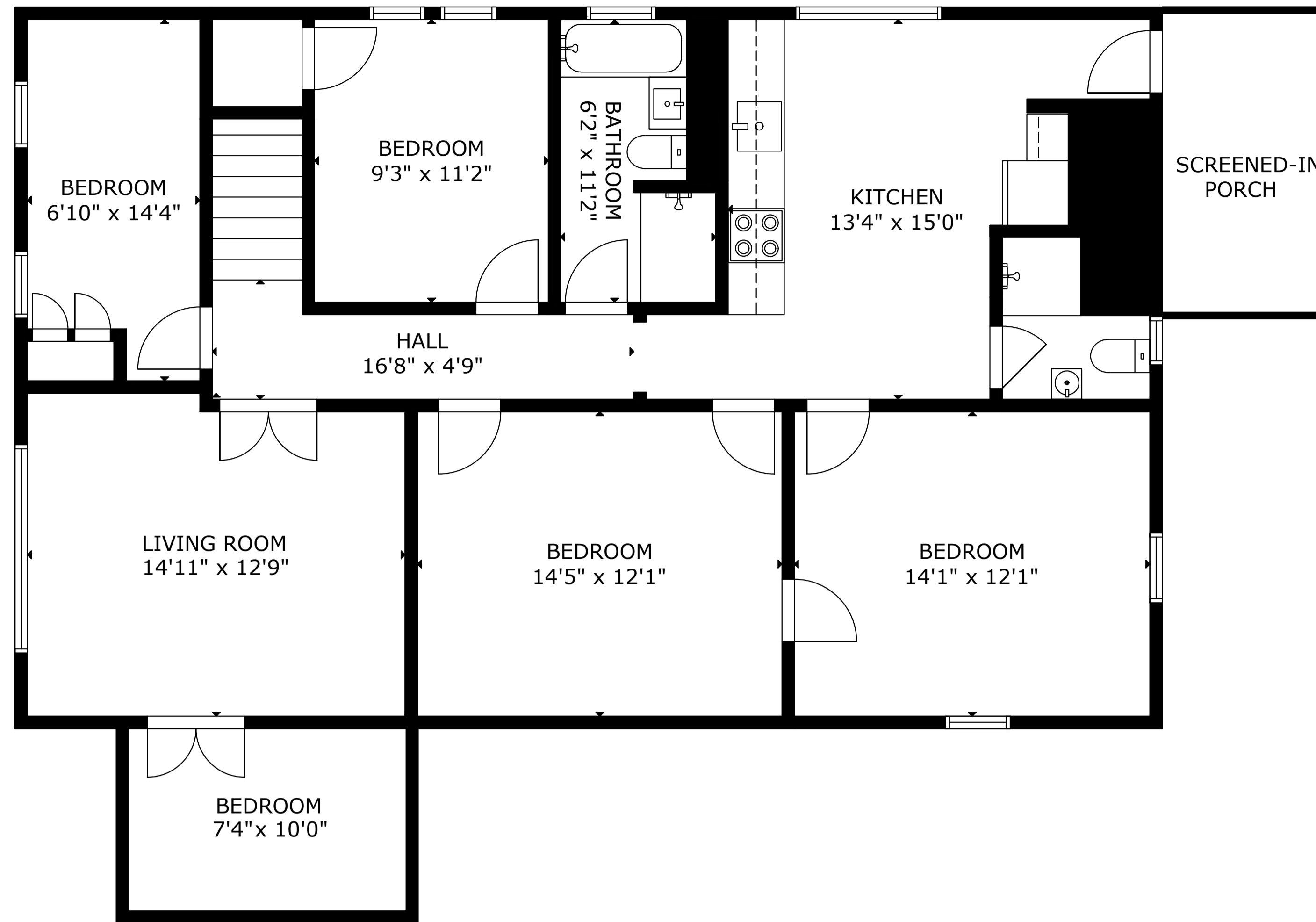
SECOND FLOOR
