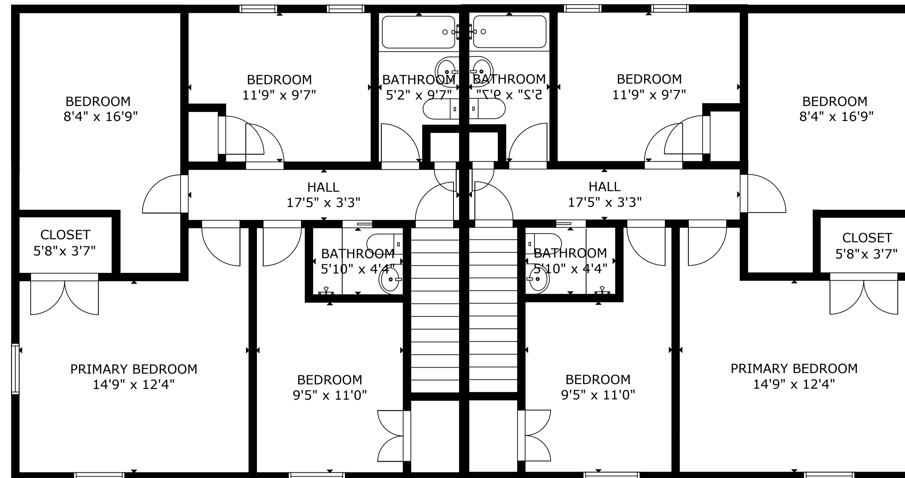
SECOND FLOOR
