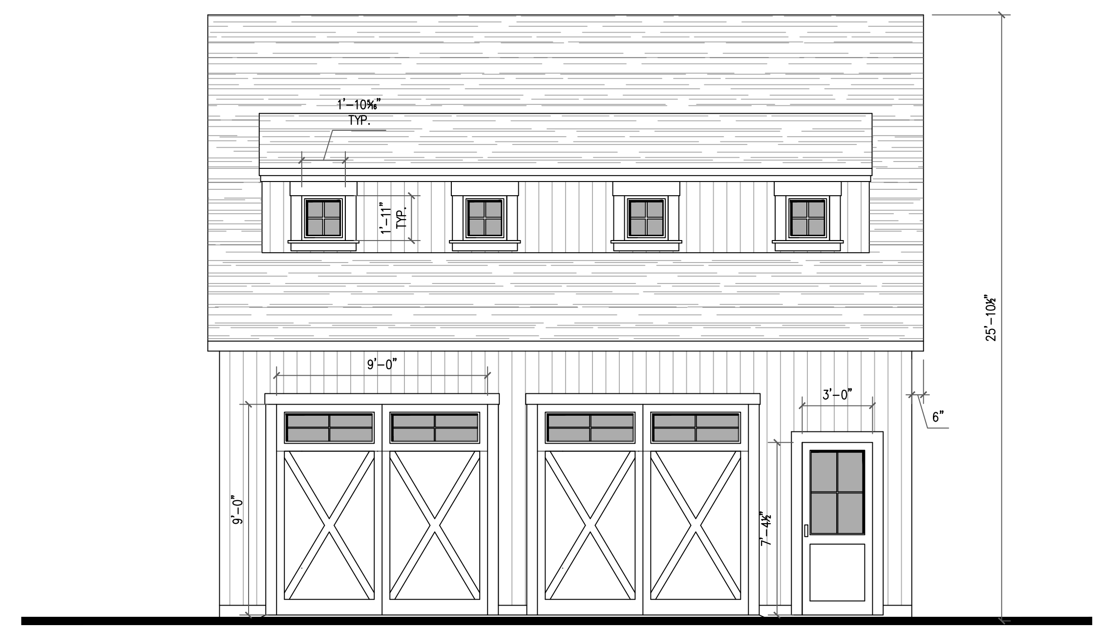
PARTIAL SOUTH ELEVATION@ GARAGE
