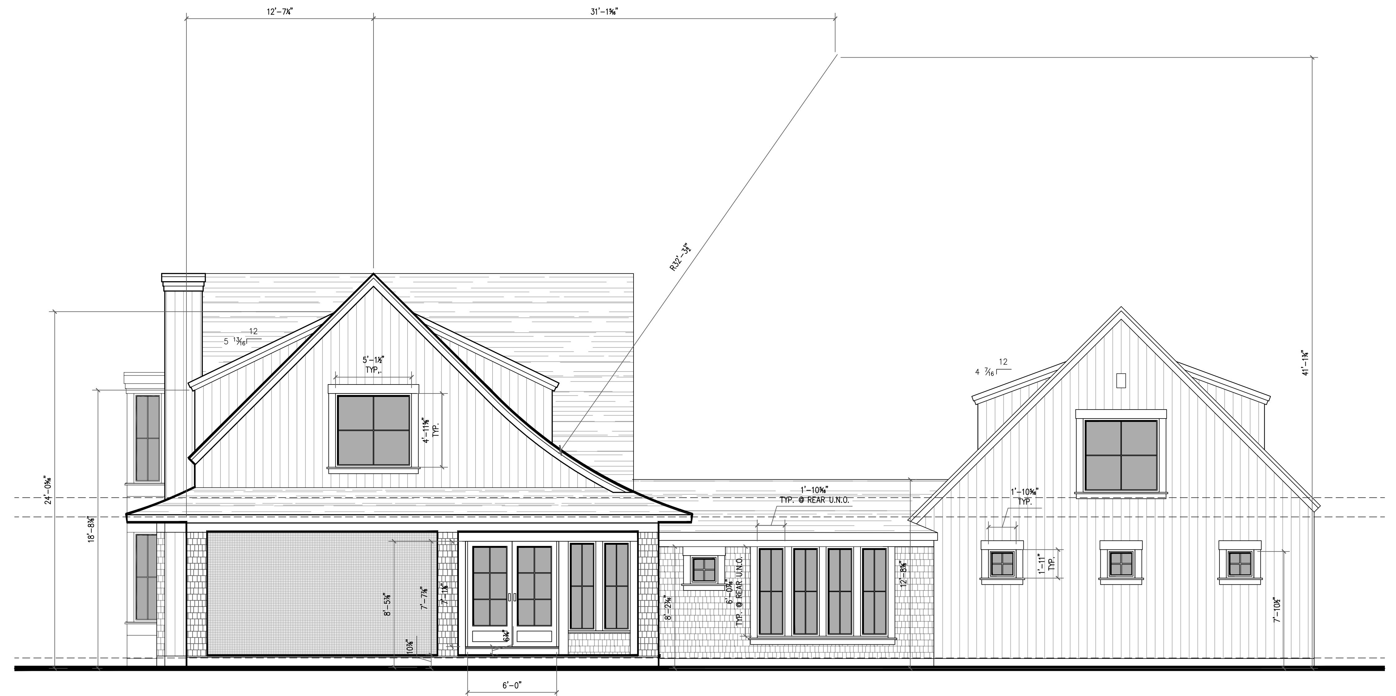
WEST ELEVATION
